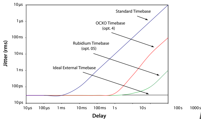
Jitter vs. programmed delay
